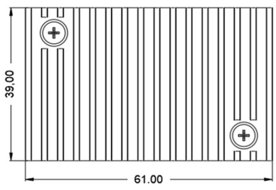
Standard+Heatsink 61.0x39.0x27.7mm
