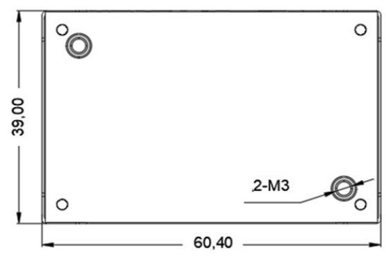
Standard 60.4x39.0x12.7mm
